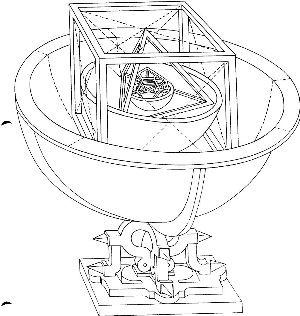
Fig. 2 Kepler's nested polyhedrons and planetary spheres ( Mysterium cosmographicum ), 1596
